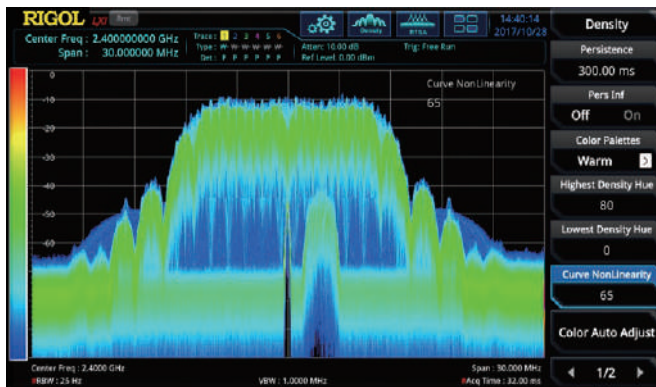
With the Density spectrum, you can find out the exceptional signals hidden behind the high-level signals, and capture them accurately with the FMT.
